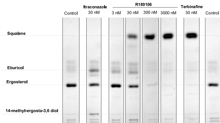
Figure 1. Trichophyton rubrum B68183 24 h sterol analysis: R189106 ( 1a ) mode of action.
